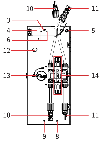
Right View
