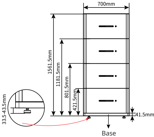
Battery group dimensions (ground installation)
