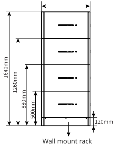
Battery group dimensions (wall-mount installation)
